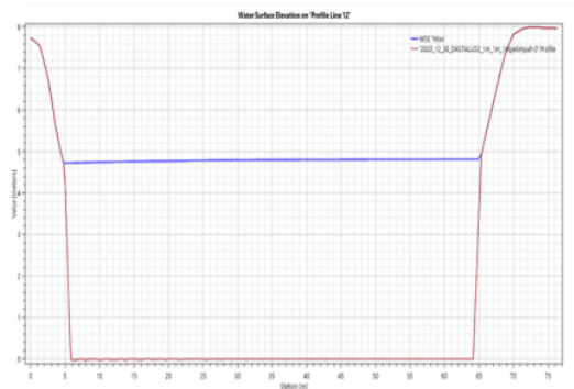
Gambar 7. Longitudinal Piece of Retention Pond Spillway
