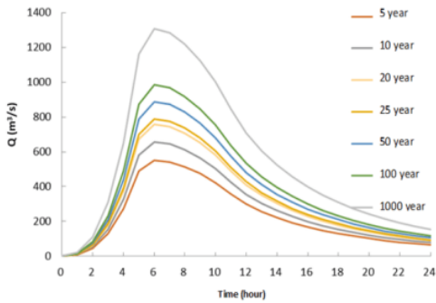
Figure 3. Mangalarang Sub-watershed Flood Hydrograph with Nakayasu Method
